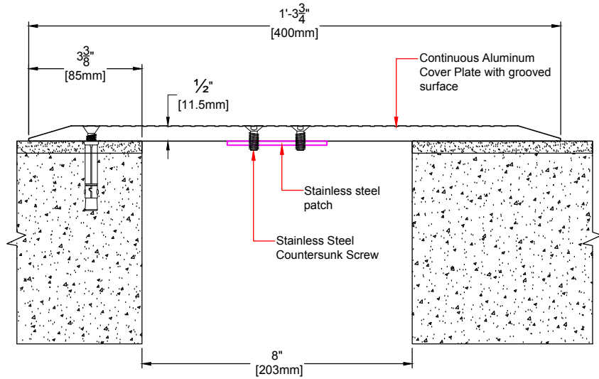
CROSS SECTION SPLICING DETAIL
