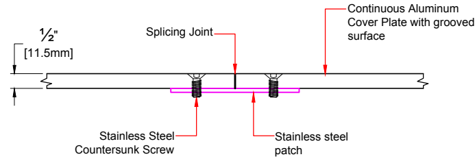
LONGITUDINAL SECTION SPLICING DETAIL
