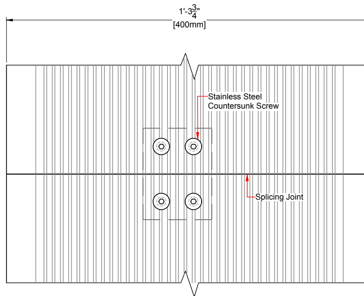
TOP-PLATE SPLICING DETAIL
