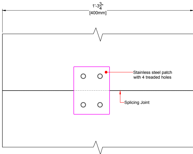
BOTTOM-PLATE SPLICING DETAIL
