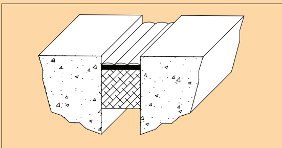
Fig.6 (COMPLETE INSTALLATION)
